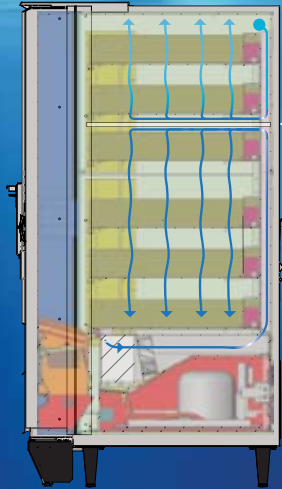
Patented air flow design allows for frozen and refrigerated (split) zones even in hot climates.
