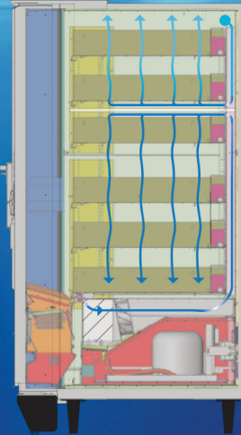
Patented air flow design allows for frozen and refrigerated (split) zones even in hot climates.
